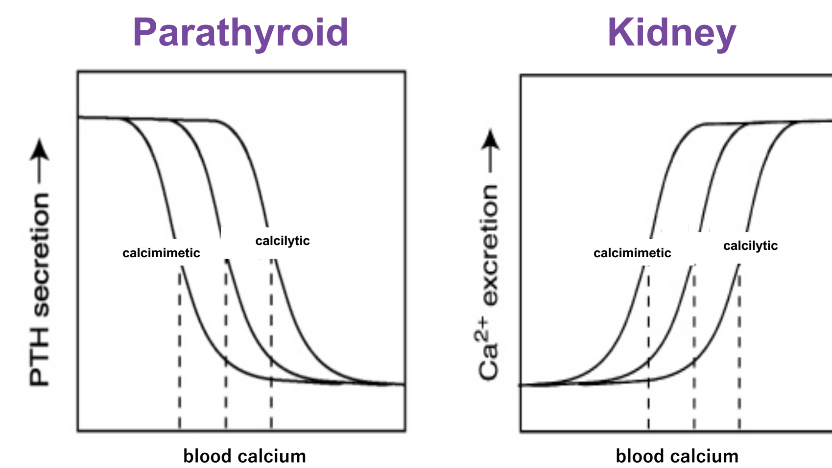
Figure 2: The effects of allosteric modulators on the CaSR Calcilytics decrease the sensitivity of CaSRs to extracellular calcium, resulting in increased PTH secretion (left panel) and decreased calcium excretion (right panel). Calcimimetics have the opposite effect.
